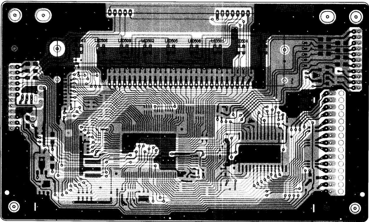
Bottom View
